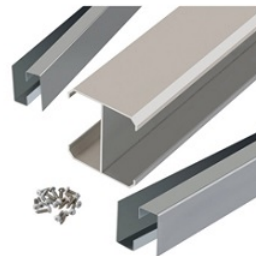
Dover Fence Wind Kit with post stiffener Model # 149051
